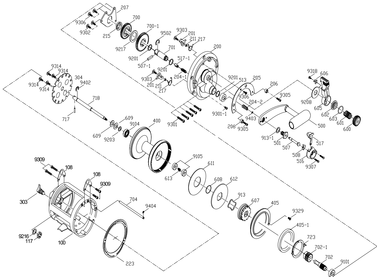
T - 30 - II (1 of 2) Spare Parts
